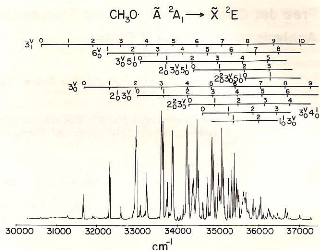
Figure 2. Laser excitation spectrum of \text{CH}_3\text{O} . The vibrational assignments are indicated above. Only one hot-band sequence, 3_1^1 , could be detected and it only weakly, indicating that the radical is relatively cold vibrationally as well as rotationally.
