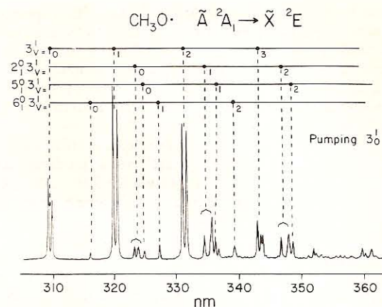
Figure 3. Laser-excited, wavelength-resolved emission spectrum of CH 3 O using a monochromator and OMA. The assignments of the main peaks are indicated above the trace. The pump laser frequency coincides with the 3 0 1 excitation band. The OMA is gated open for 3.6 \mu s and delayed by 0.6 \mu s from the probe laser's firing. In this way scattered laser light is rejected and the emission lines near the laser pump frequency maintain their appropriate relative intensity with respect to the remainder of the spectrum. The monochromator slit width is 150 \mu m yielding an effective spectral resolution of \approx 15 cm -1 . A total of 12 000 laser pulses (10 min real time) was integrated to obtain the trace.
