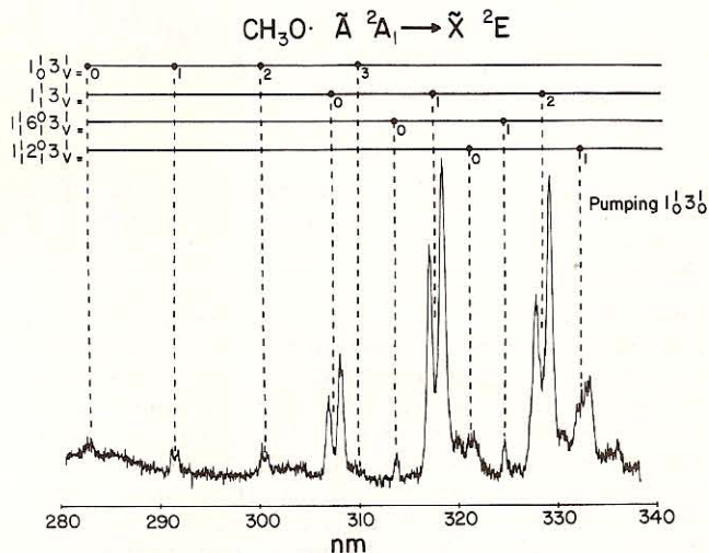
Figure 5. Laser-excited, wavelength-resolved emission spectrum of CH 3 O observed when the band 1 0 3 0 1 is pumped. The other experimental conditions are as in Figure 4.
