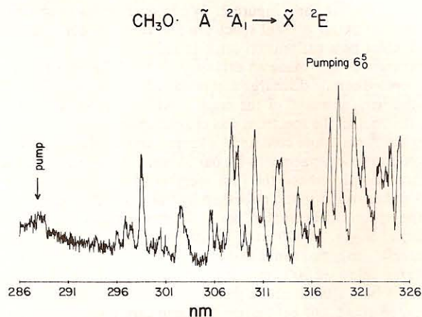
Figure 4. Laser-excited, wavelength-resolved emission spectrum of CH 3 O. The pump frequency coincides with the band assigned as 6 0 5 . The remaining experimental conditions are as in Figure 3, except the monochromator slit width has been widened to 500 \mu m and the integration time shortened to 8 min. No vibrational assignments have yet been made for this spectrum.
