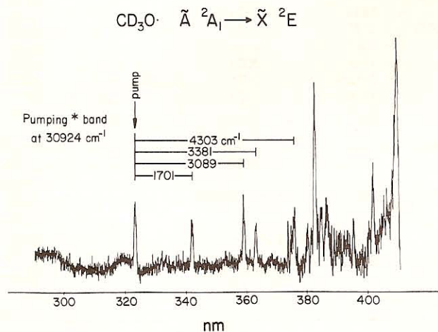
Figure 7. Laser-excited, wavelength-resolved emission spectrum of \text{CD}_3\text{O} observed when the 30924 "starred" band of Figure 6 is excited. Other conditions are the same as in Figure 3, except the monochromator slit width is 1 mm.
