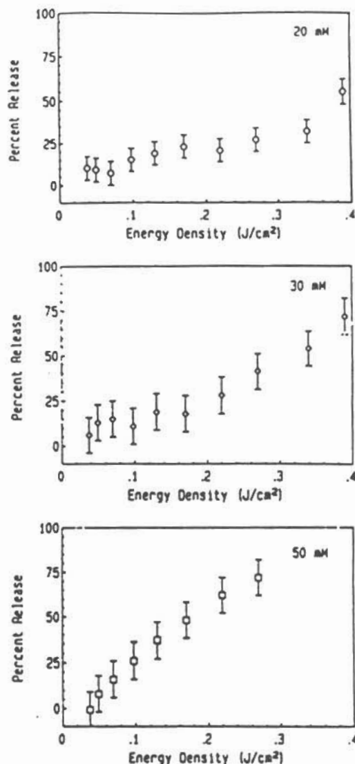
Figure 4. Effects of a single 25 ps laser pulse at 532 nm on release of sulforhodamine dye from 2.2 \mu\text{m} diameter liposomes as a function of energy density. (a) 20 mM (b) 30 mM and (c) 50 mM sulforhodamine dye.
