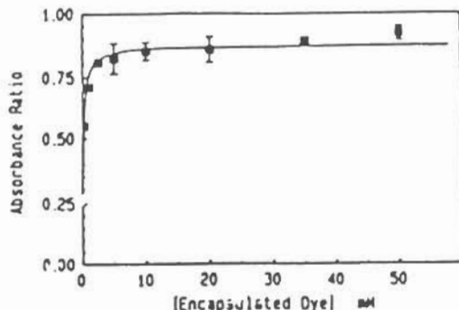
Figure 2. Ratio of dimer to monomer absorbance as a function of the encapsulated dye concentration in the liposome.
