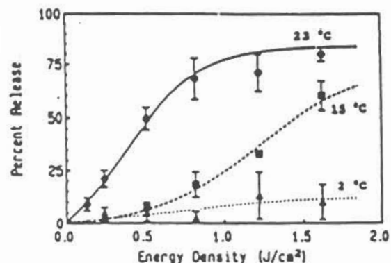
Figure 6. Effect of initial temperature on the single 8 ns laser pulse induced release of contents of 4.5 \mu\text{m} diameter liposomes with 50 mM sulforhodamine.
