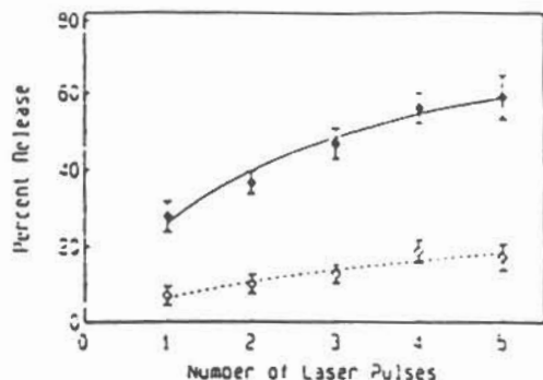
Figure 7. Effects of irradiating 2.2 \mu\text{m} diameter liposomes containing 20 mM sulforhodamine with multiple 8 ns laser pulses at 532 nm. Open and solid symbols refer to 0.8 \text{J}/\text{cm}^2 and 1.7 \text{J}/\text{cm}^2 pulses, respectively. There was about 1 s delay between sequential pulses.
