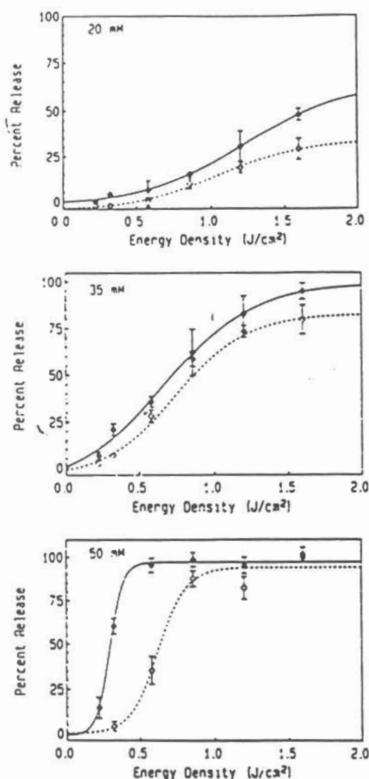
Figure 3. Effects of a single 8 ns laser pulse at 532 nm on release of sulforhodamine dye from liposomes as a function of energy density. Open and solid symbols refer to 2 \mu\text{m} and 4.5 \mu\text{m} diameter liposomes, respectively. (a) 20 mM (b) 35 mM and (c) 50 mM sulforhodamine dye.
