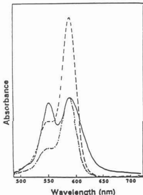
Figure 1. Absorption spectrum of 20 mM sulforhodamine encapsulated in liposomes (solid curve); spectrum of the dye after thermal release (dashed curve); spectrum of released dye normalized at the point of maximum absorbance (dash-dot curve).
