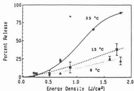
Figure 5. Effect of initial temperature on the single 8 ns laser pulse induced release of contents 2 \mu\text{m} diameter liposomes with 50 mM sulforhodamine.
